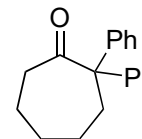
2,2-diphenylcycloheptanone ( 2 ) 13 C NMR (100 MHz, CDCl 3 )
